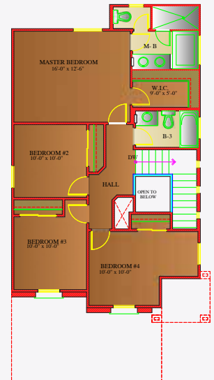
2ND. FLOOR PLAN NOT TO SCALE
